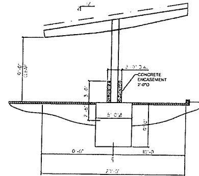
FRAME CROSS SECTION
